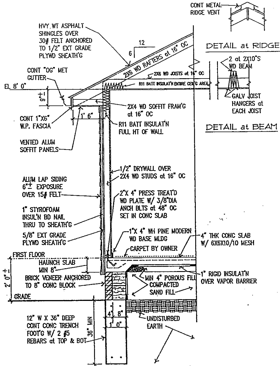
SECTION thru TYPICAL SIDEWALL
