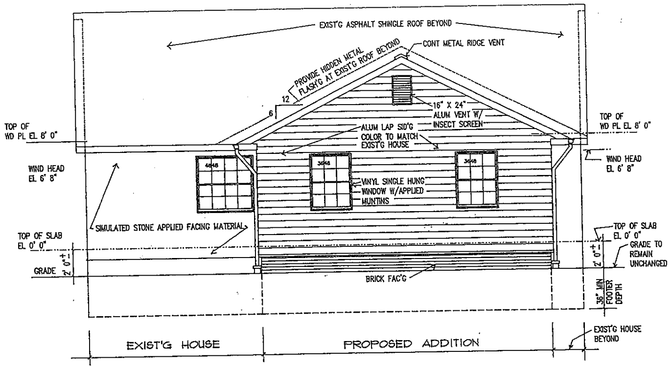
WEST (REAR) ELEVATION
