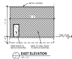
EAST ELEVATION 1" = 1' - 0"
