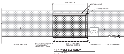
WEST ELEVATION 1" = 1' - 0"
