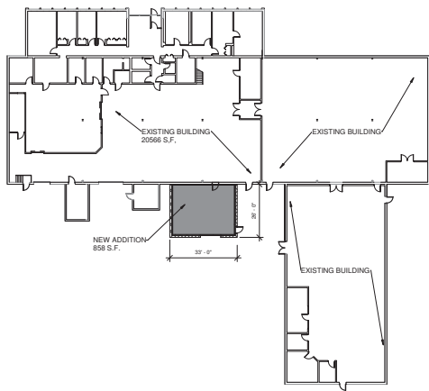
OVERALL BUILDING PLAN 1" = 30' - 0"
